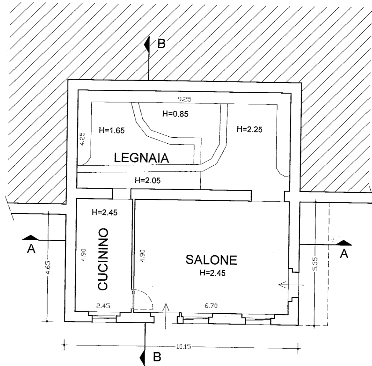
PIANO SEMINTERRATO
